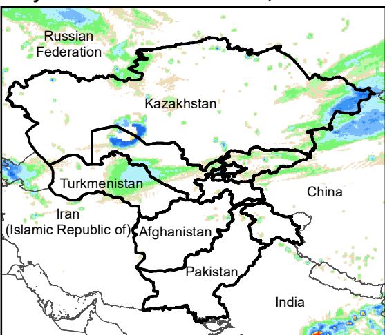
Daily Rainfall estimate for 6 Oct., 2020
