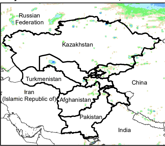
Daily Rainfall estimate for 15 Oct., 2020
