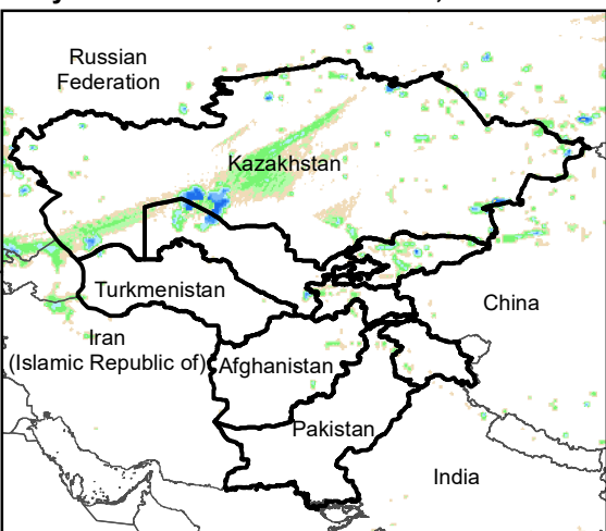
Daily Rainfall estimate for 21 Oct., 2020
