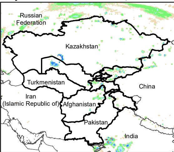
Daily Rainfall estimate for 22 Oct., 2020
