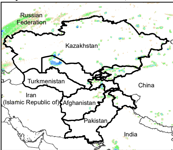
Daily Rainfall estimate for 23 Oct., 2020
