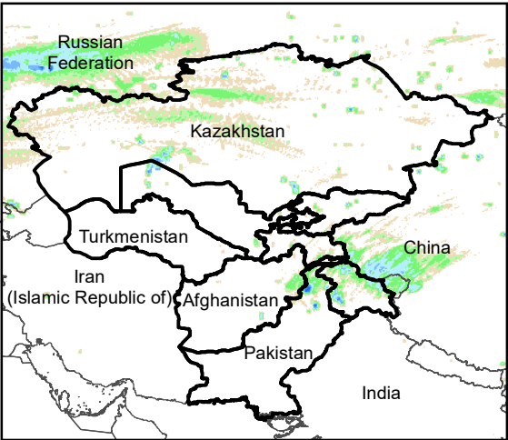
Daily Rainfall estimate for 25 Oct., 2020
