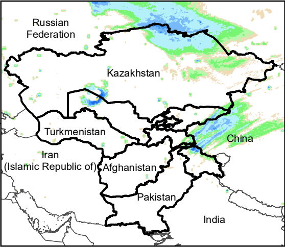
Daily Rainfall estimate for 1 Nov., 2020
