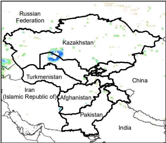
Daily Rainfall estimate for 2 Nov., 2020
