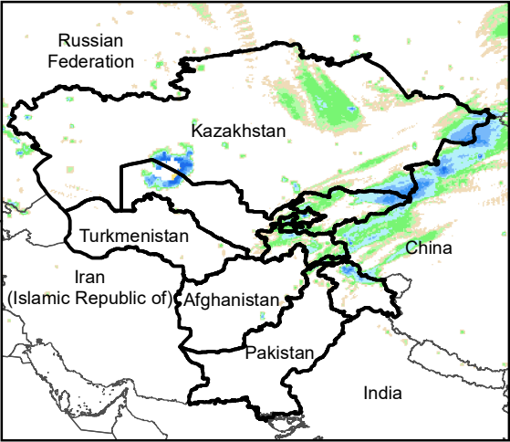
Daily Rainfall estimate for 31 Oct., 2020
