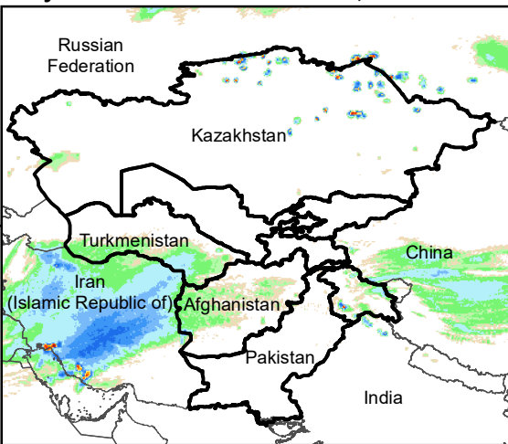
Daily Rainfall estimate for 9 Dec., 2020
