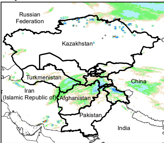
Daily Rainfall estimate for 10 Dec., 2020
