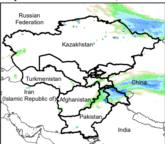
Daily Rainfall estimate for 8 Dec., 2020
