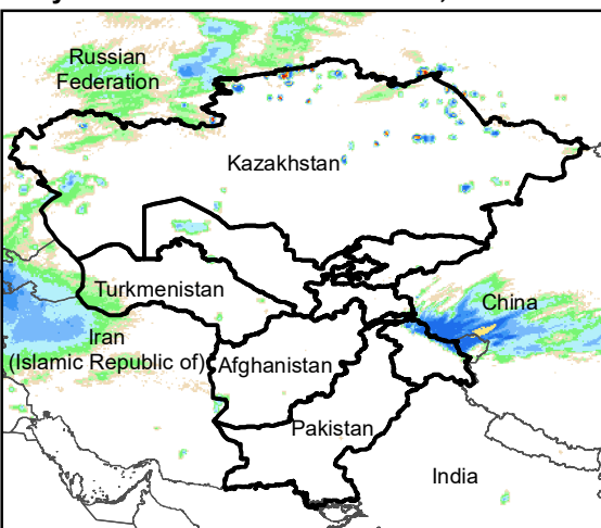
Daily Rainfall estimate for 16 Dec., 2020
