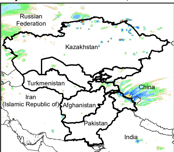
Daily Rainfall estimate for 15 Dec., 2020
