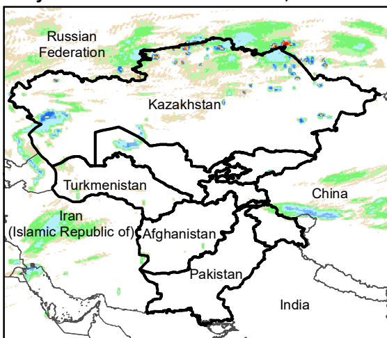
Daily Rainfall estimate for 17 Dec., 2020
