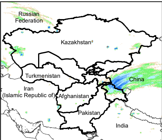
Daily Rainfall estimate for 6 Jan., 2021
