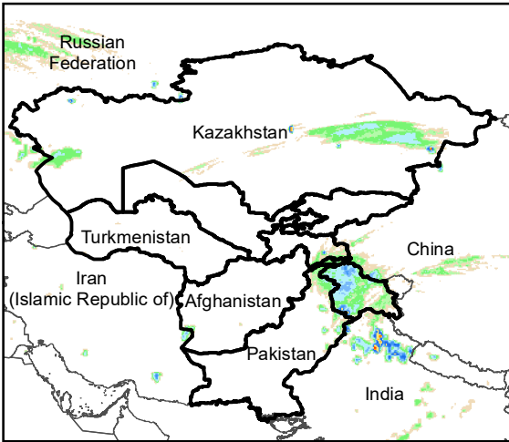
Daily Rainfall estimate for 8 Jan., 2021
