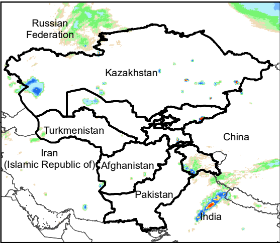
Daily Rainfall estimate for 6 Jan., 2021
