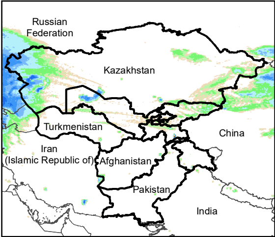
Daily Rainfall estimate for 16 Jan., 2021
