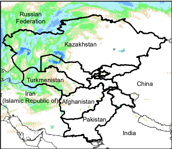
Daily Rainfall estimate for 15 Jan., 2021
