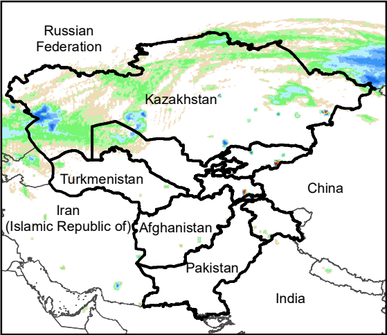
Daily Rainfall estimate for 14 Jan., 2021
