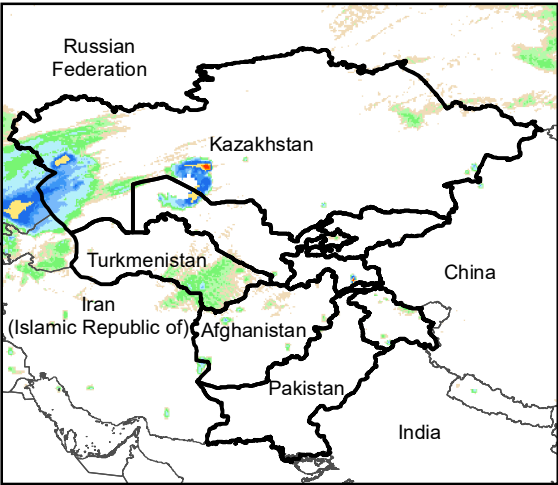
Daily Rainfall estimate for 17 Jan., 2021
