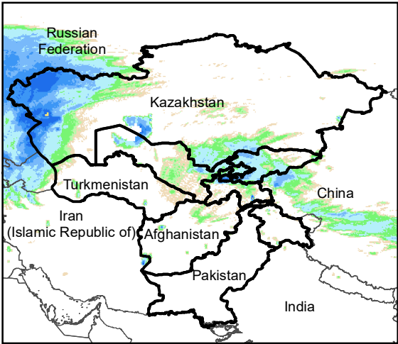
Daily Rainfall estimate for 18 Jan., 2021
