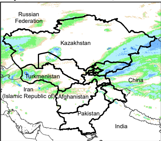
Daily Rainfall estimate for 8 Mar., 2021
