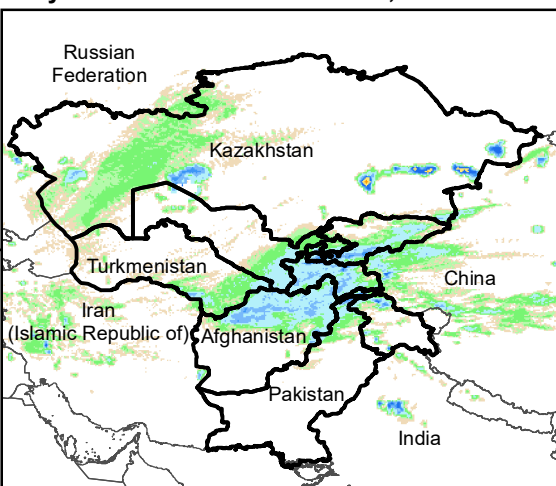
Daily Rainfall estimate for 9 Mar., 2021
