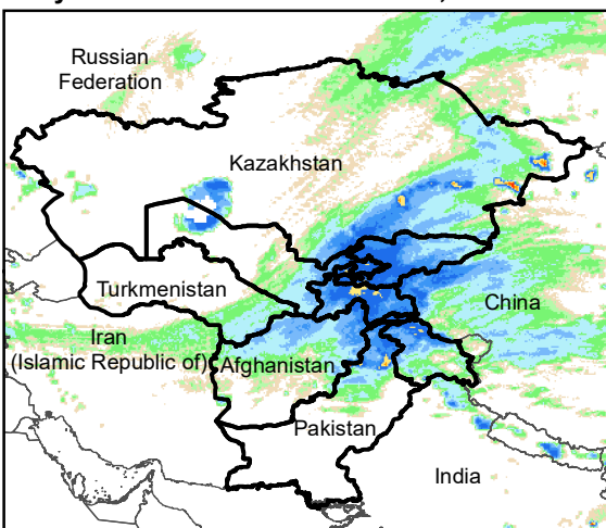
Daily Rainfall estimate for 10 Mar., 2021
