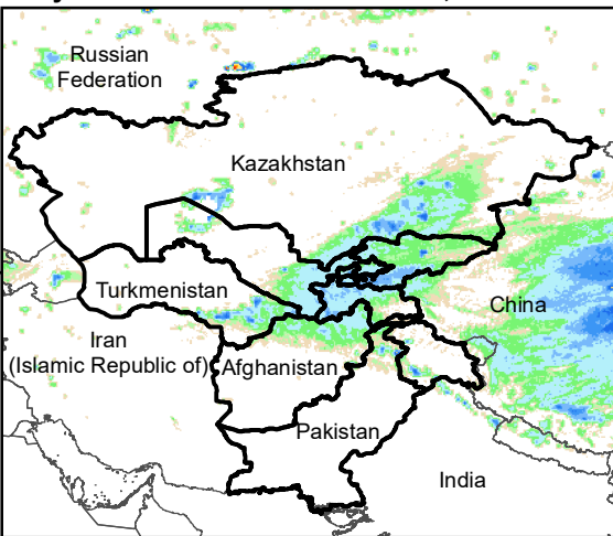
Daily Rainfall estimate for 30 Mar., 2021
