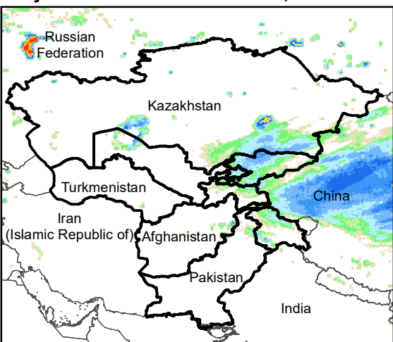
Daily Rainfall estimate for 29 Mar., 2021
