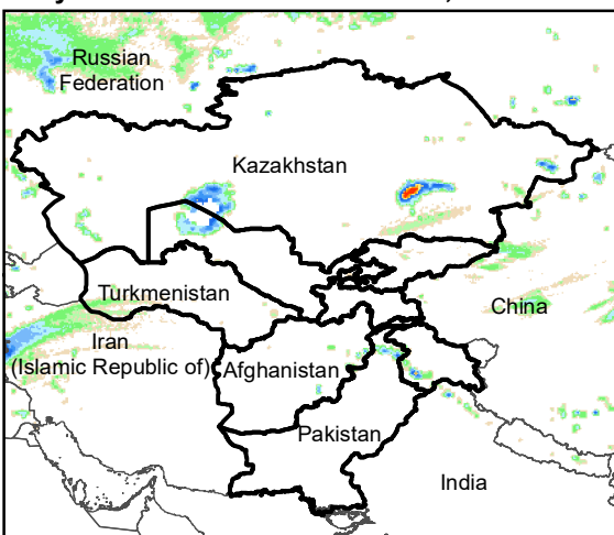
Daily Rainfall estimate for 31 Mar., 2021
