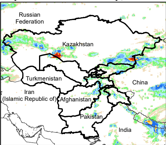
Daily Rainfall estimate for 31 May., 2021
