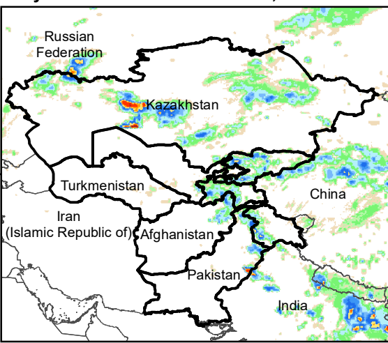
Daily Rainfall estimate for 1 Jun., 2021
