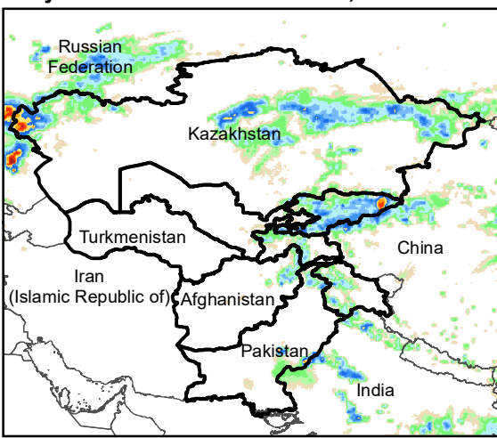
Daily Rainfall estimate for 2 Jun., 2021
