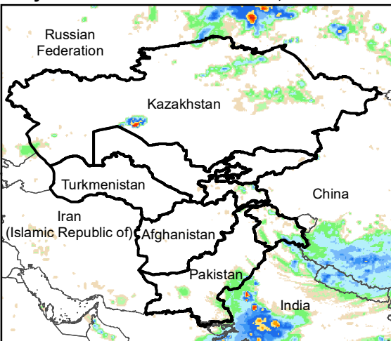
Daily Rainfall estimate for 28 Jul., 2021
