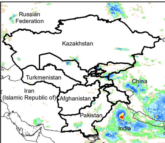
Daily Rainfall estimate for 21 Aug., 2021
