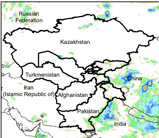
Daily Rainfall estimate for 22 Aug., 2021
