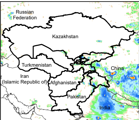
Daily Rainfall estimate for 20 Aug., 2021
