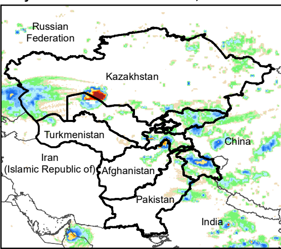
Daily Rainfall estimate for 4 Oct., 2021
