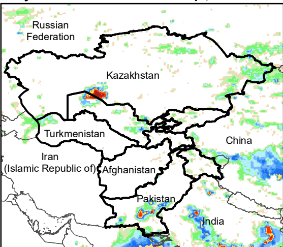
Daily Rainfall estimate for 3 Oct., 2021
