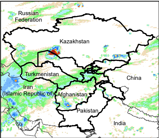
Daily Rainfall estimate for 9 Mar., 2023
