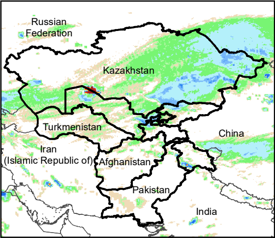
Daily Rainfall estimate for 8 Mar., 2023
