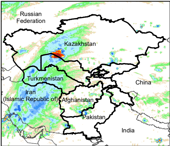
Daily Rainfall estimate for 10 Mar., 2023
