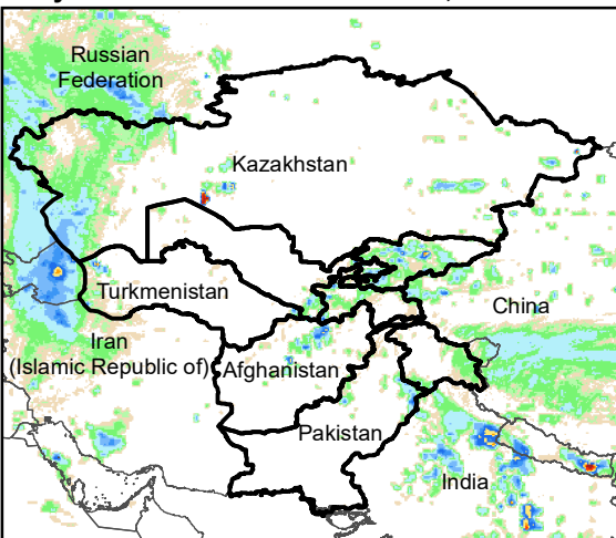
Daily Rainfall estimate for 3 Apr., 2023
