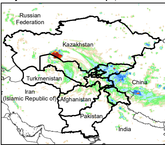
Daily Rainfall estimate for 4 Apr., 2023
