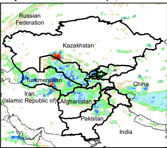
Daily Rainfall estimate for 2 Apr., 2023
