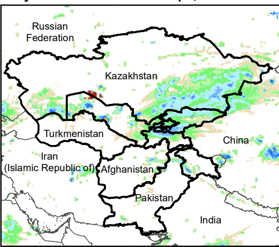
Daily Rainfall estimate for 7 Apr., 2023
