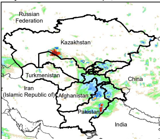
Daily Rainfall estimate for 8 Apr., 2023
