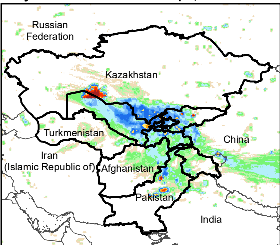
Daily Rainfall estimate for 6 Apr., 2023
