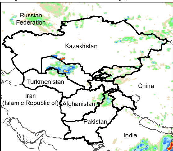
Daily Rainfall estimate for 2 Oct., 2023
