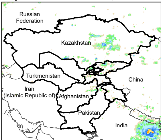
Daily Rainfall estimate for 4 Oct., 2023
