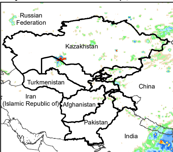
Daily Rainfall estimate for 3 Oct., 2023
