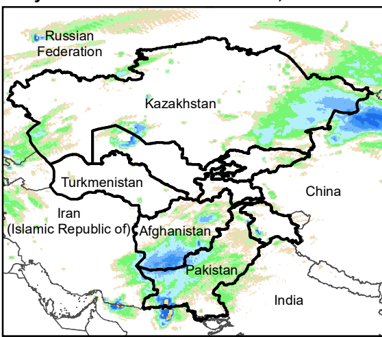
Daily Rainfall estimate for 25 Nov., 2023
