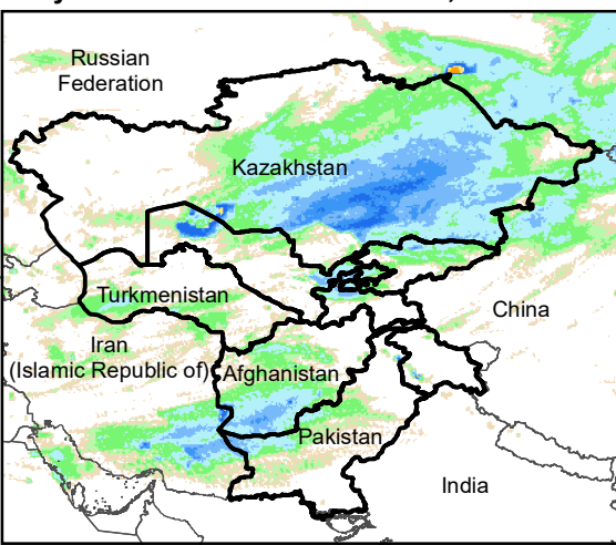
Daily Rainfall estimate for 24 Nov., 2023
