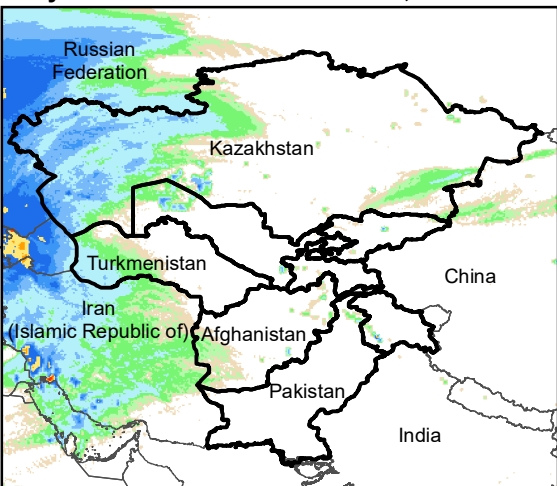
Daily Rainfall estimate for 23 Nov., 2023
