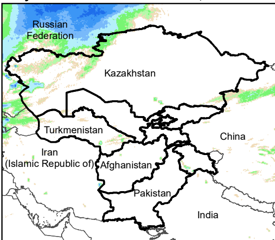
Daily Rainfall estimate for 20 Jan., 2024
