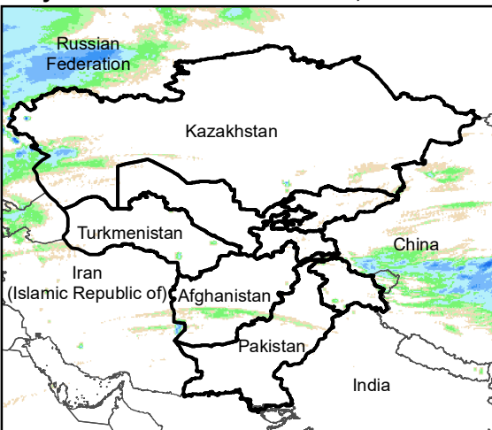
Daily Rainfall estimate for 19 Jan., 2024
