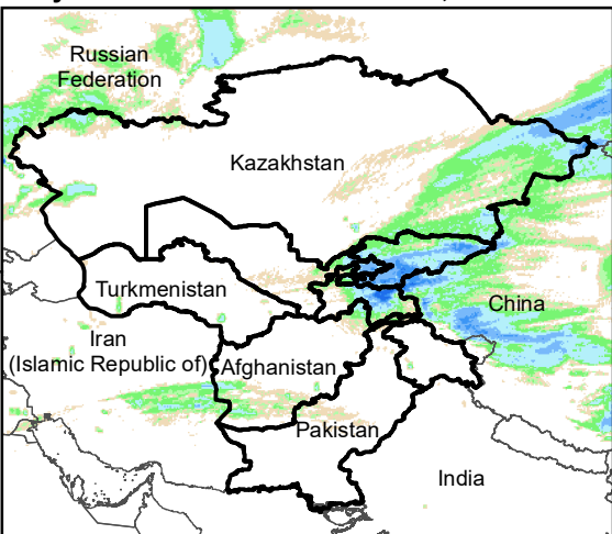
Daily Rainfall estimate for 18 Jan., 2024
