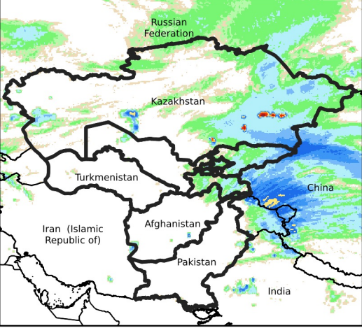
Daily Rainfall estimate for Feb 4, 2024
