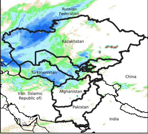
Daily Rainfall estimate for Feb 6, 2024
