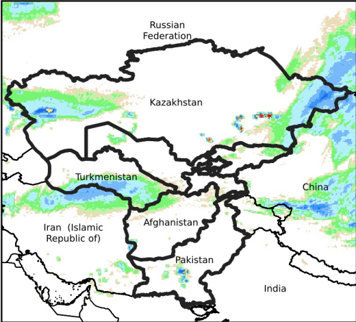
Daily Rainfall estimate for Feb 5, 2024
