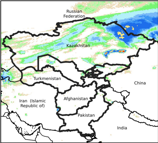
Daily Rainfall estimate for Feb 12, 2024
