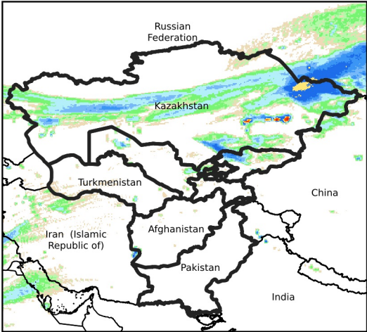
Daily Rainfall estimate for Feb 13, 2024
