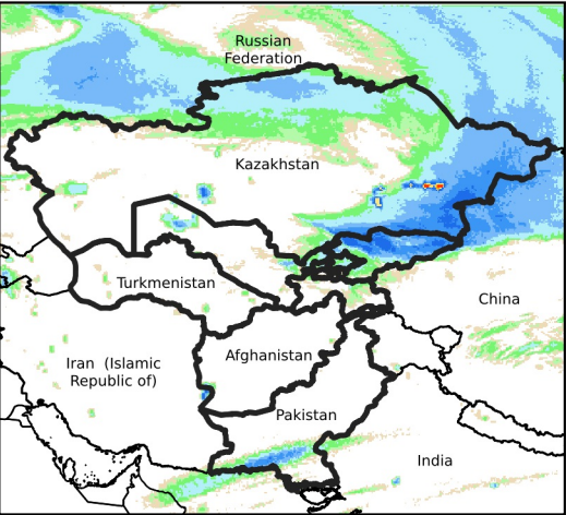
Daily Rainfall estimate for Feb 11, 2024
