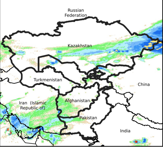
Daily Rainfall estimate for Feb 11, 2024
