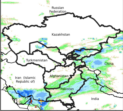
Daily Rainfall estimate for Feb 12, 2024
