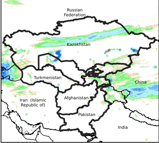
Daily Rainfall estimate for Mar 7, 2024
