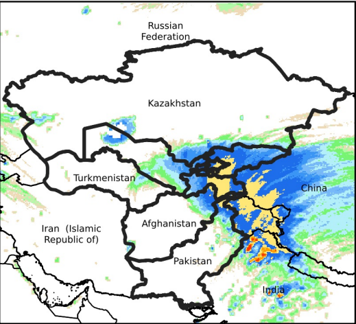
Daily Rainfall estimate for Mar 5, 2024
