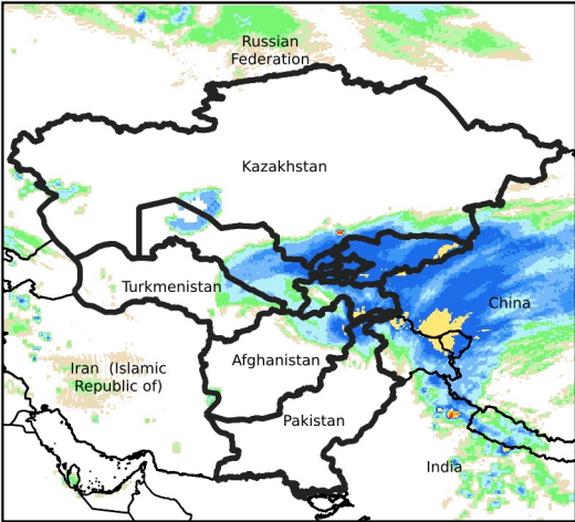
Daily Rainfall estimate for Mar 6, 2024
