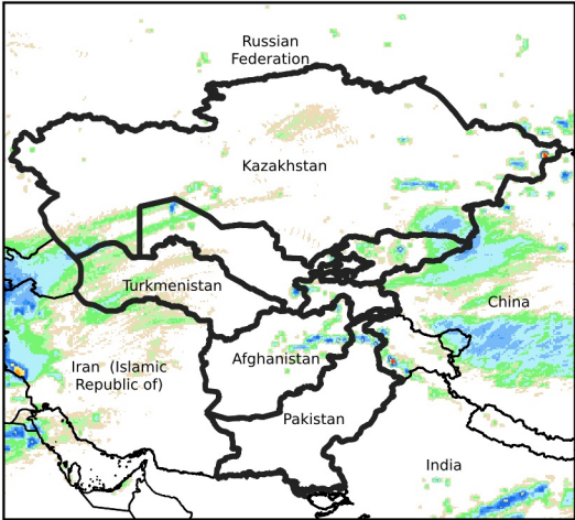
Daily Rainfall estimate for Apr 10, 2024
