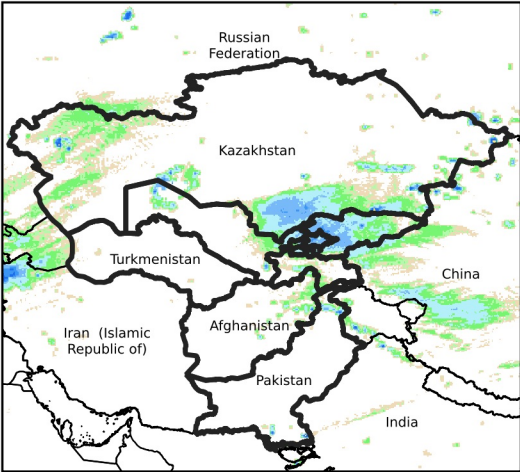
Daily Rainfall estimate for Apr 9, 2024
