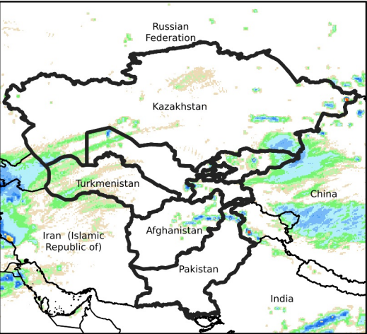
Daily Rainfall estimate for Apr 10, 2024
