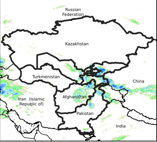
Daily Rainfall estimate for Apr 21, 2024
