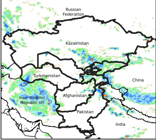
Daily Rainfall estimate for Apr 23, 2024
