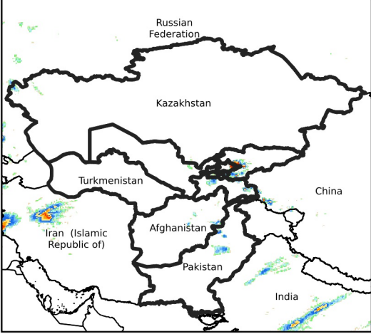
Daily Rainfall estimate for Apr 22, 2024
