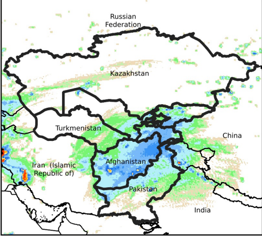
Daily Rainfall estimate for May 3, 2024
