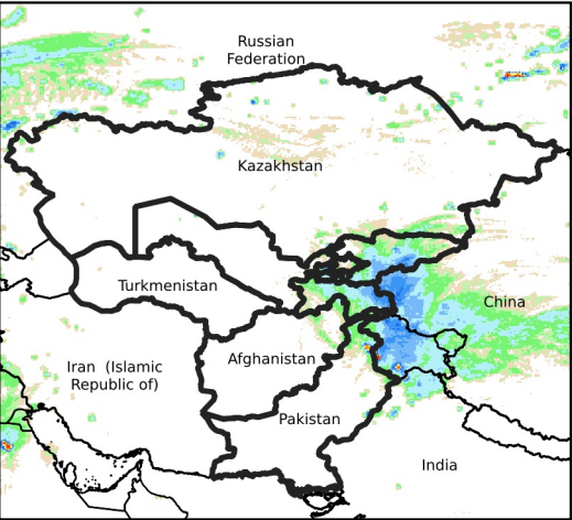
Daily Rainfall estimate for May 2, 2024
