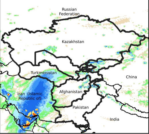
Daily Rainfall estimate for May 2, 2024
