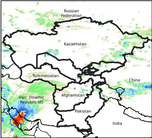
Daily Rainfall estimate for May 4, 2024
