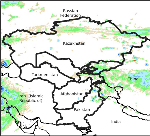
Daily Rainfall estimate for May 3, 2024
