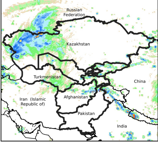
Daily Rainfall estimate for May 8, 2024
