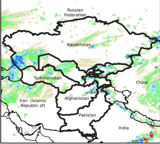
Daily Rainfall estimate for May 7, 2024
