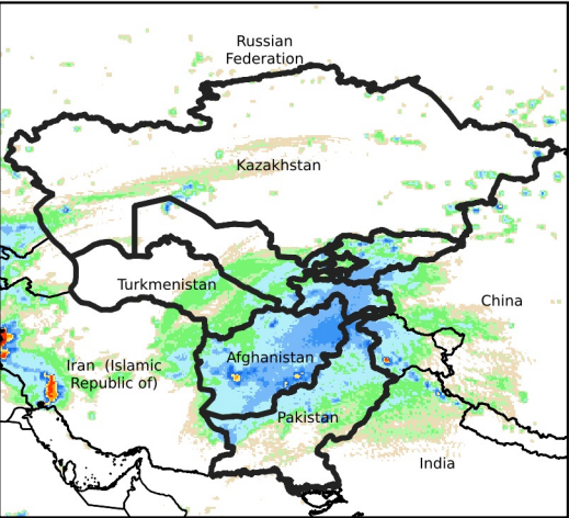
Daily Rainfall estimate for May 6, 2024
