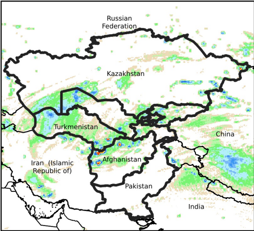
Daily Rainfall estimate for May 7, 2024
