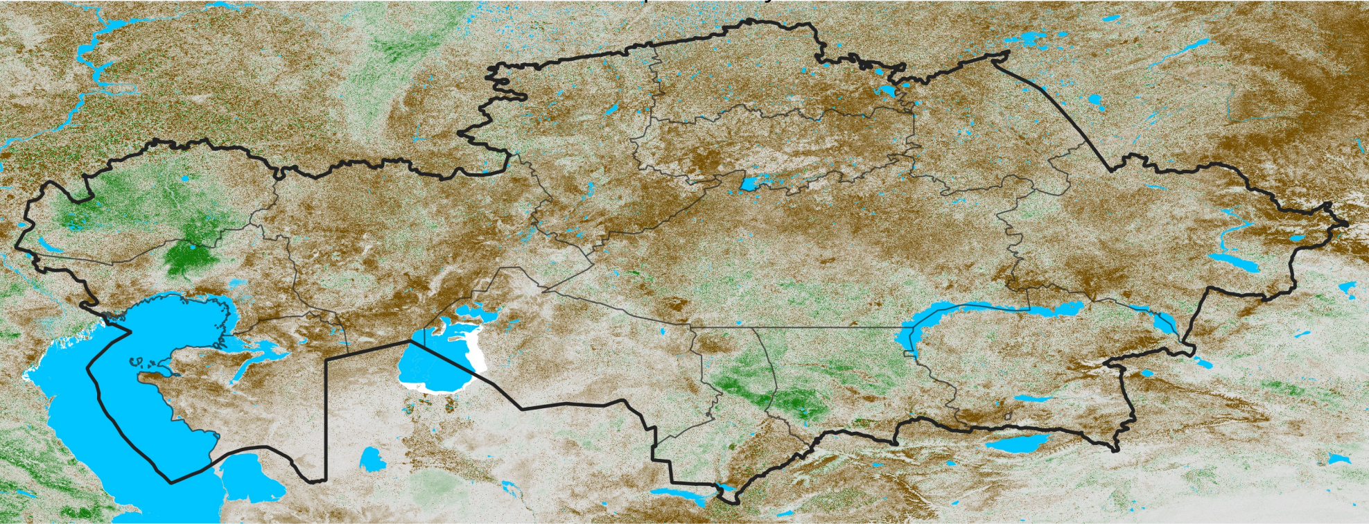
NDVI Difference
