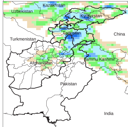
Daily Precip. Forecast for 23 Feb., 2009
