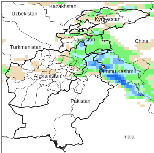
Daily Precip. Forecast for 21 Feb., 2009
