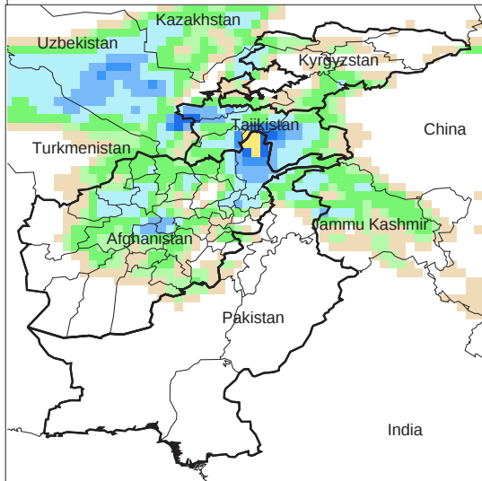
Daily Precip. Forecast for 22 Feb., 2009
