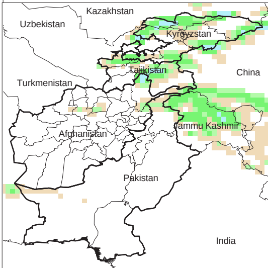
Daily Precip. Forecast for 26 Feb., 2009
