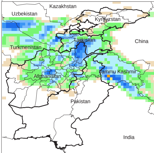
Daily Precip. Forecast for 25 Feb., 2009
