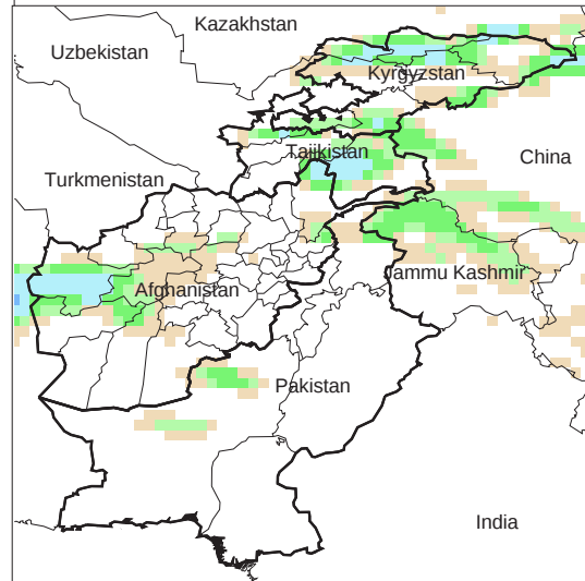
Daily Precip. Forecast for 27 Feb., 2009
