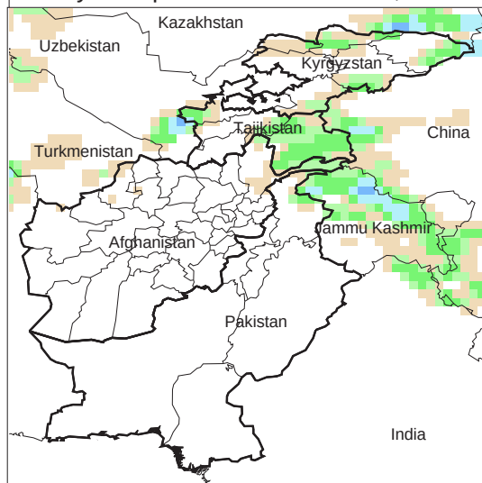
Daily Precip. Forecast for 4 Mar., 2009
