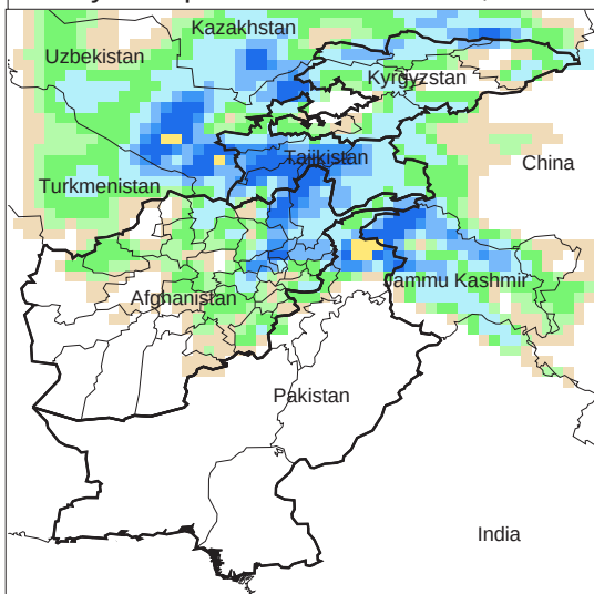
Daily Precip. Forecast for 3 Mar., 2009
