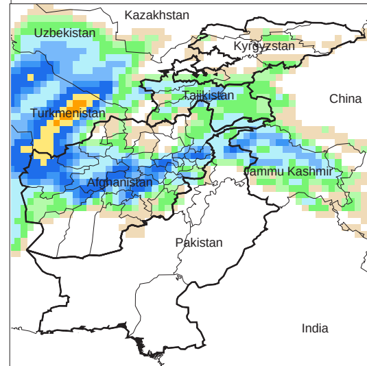
Daily Precip. Forecast for 5 Mar., 2009
