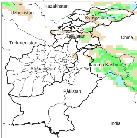
Daily Precip. Forecast for 9 Mar., 2009
