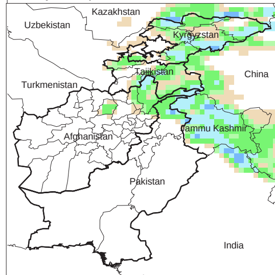
Daily Precip. Forecast for 10 Mar., 2009
