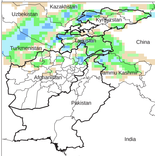
Daily Precip. Forecast for 8 Mar., 2009
