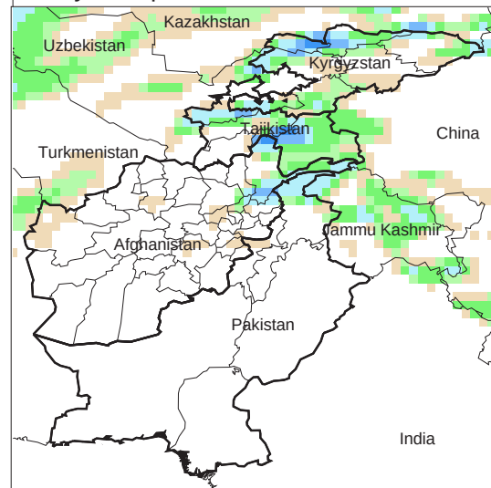
Daily Precip. Forecast for 17 Mar., 2009
