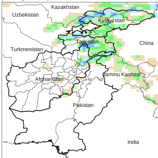
Daily Precip. Forecast for 16 Mar., 2009
