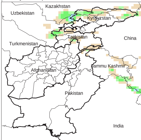
Daily Precip. Forecast for 15 Mar., 2009
