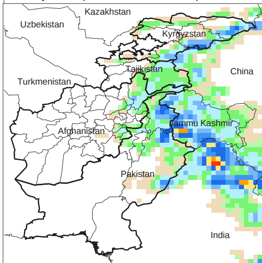
Daily Precip. Forecast for 8 Apr., 2009
