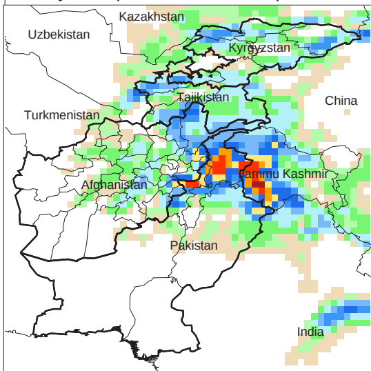
Daily Precip. Forecast for 7 Apr., 2009
