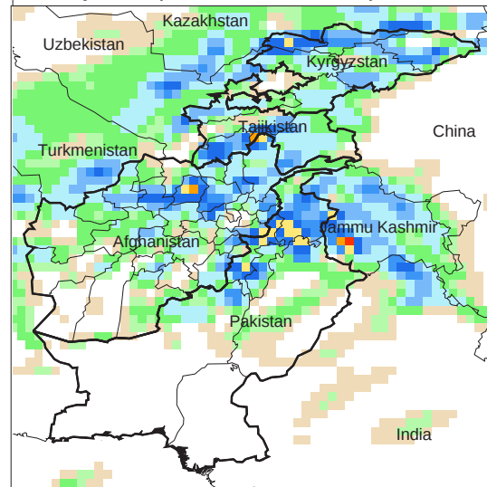
Daily Precip. Forecast for 9 Apr., 2009
