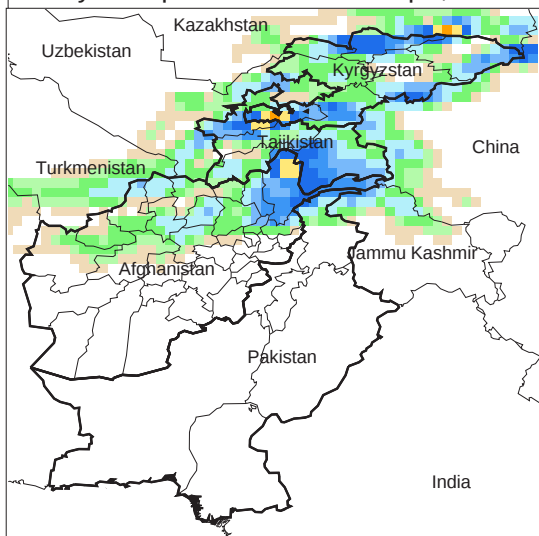
Daily Precip. Forecast for 26 Apr., 2009
