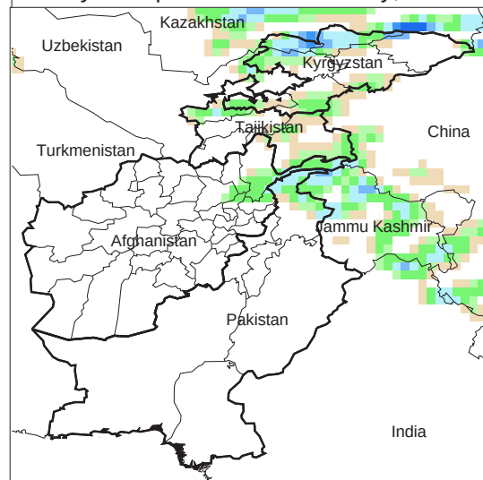
Daily Precip. Forecast for 6 May, 2009
