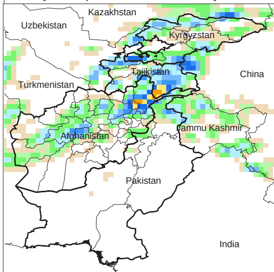
Daily Precip. Forecast for 5 May, 2009
