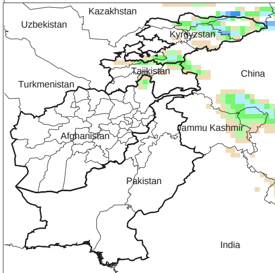
Daily Precip. Forecast for 19 May, 2009
