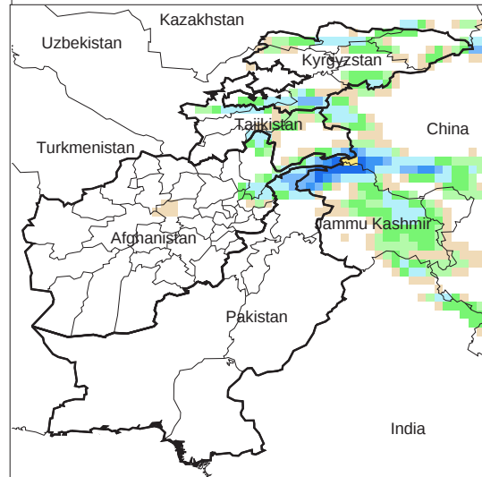
Daily Precip. Forecast for 20 May, 2009
