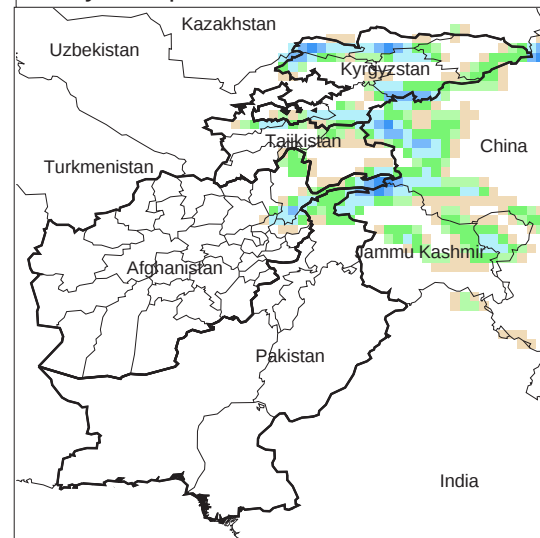
Daily Precip. Forecast for 12 Jun., 2009
