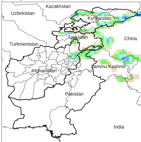
Daily Precip. Forecast for 11 Jun., 2009
