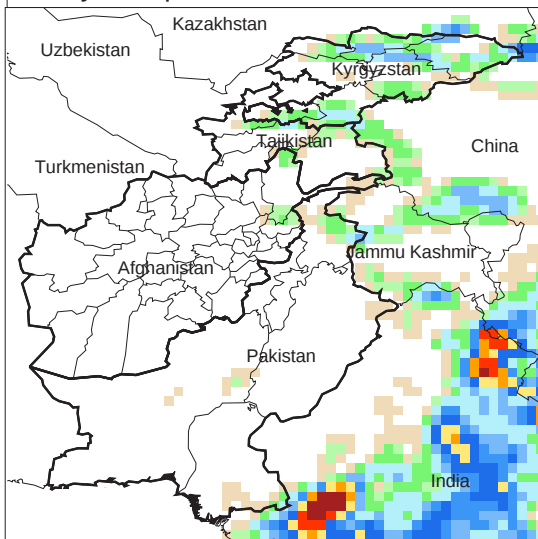
Daily Precip. Forecast for 17 Jul., 2009
