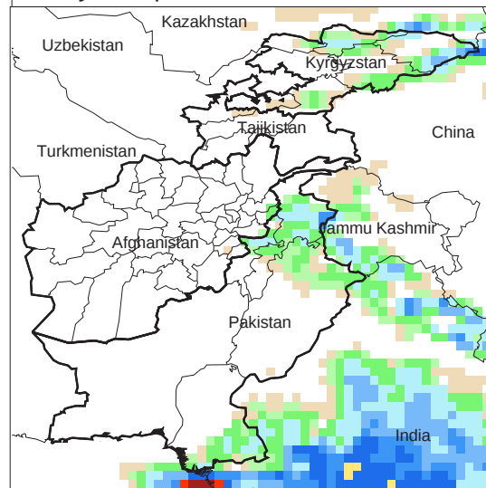
Daily Precip. Forecast for 19 Jul., 2009
