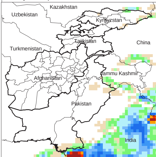
Daily Precip. Forecast for 18 Jul., 2009
