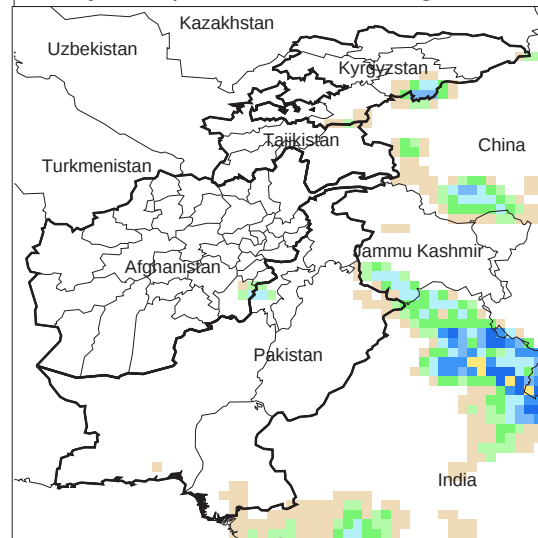
Daily Precip. Forecast for 11 Aug., 2009
