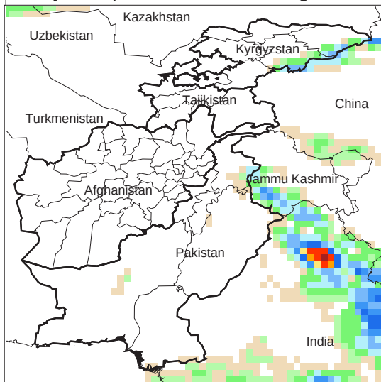
Daily Precip. Forecast for 10 Aug., 2009
