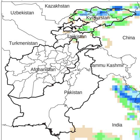
Daily Precip. Forecast for 9 Aug., 2009
