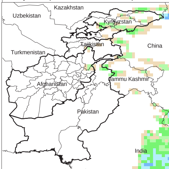
Daily Precip. Forecast for 1 Oct., 2009
