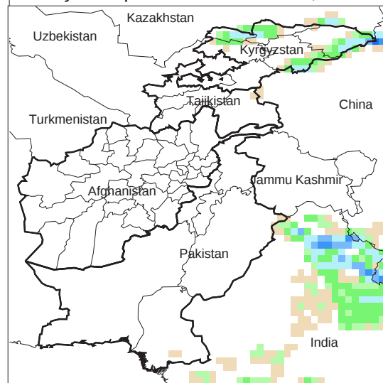
Daily Precip. Forecast for 3 Oct., 2009
