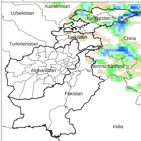
Daily Precip. Forecast for 12 Oct., 2009
