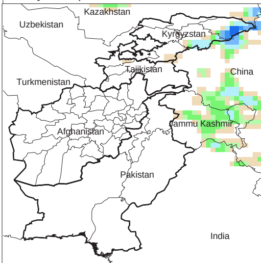
Daily Precip. Forecast for 13 Oct., 2009
