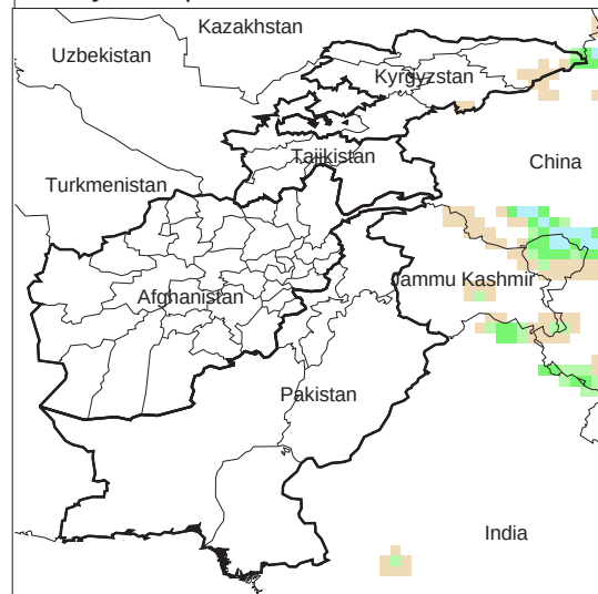
Daily Precip. Forecast for 14 Oct., 2009
