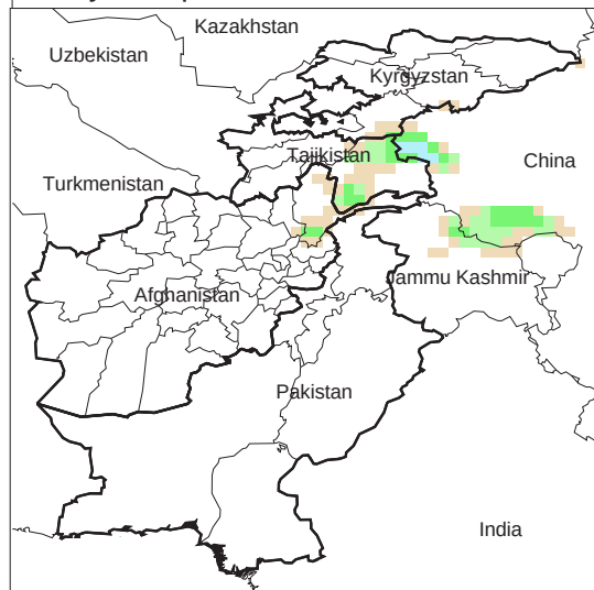
Daily Precip. Forecast for 25 Oct., 2009
