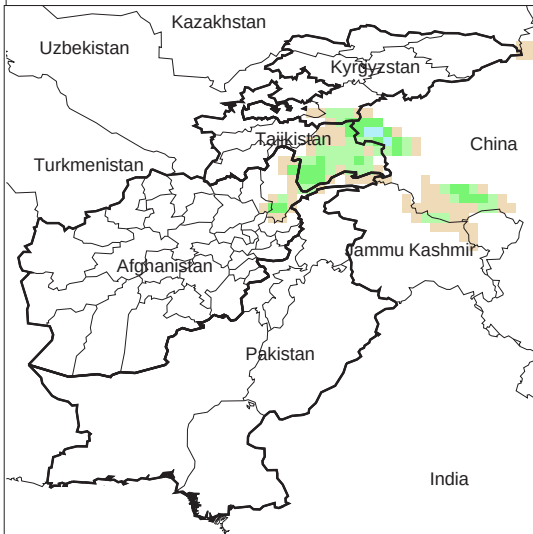
Daily Precip. Forecast for 25 Oct., 2009
