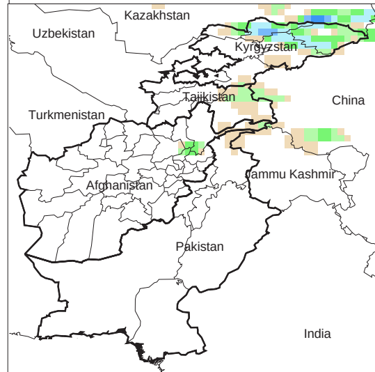
Daily Precip. Forecast for 26 Oct., 2009
