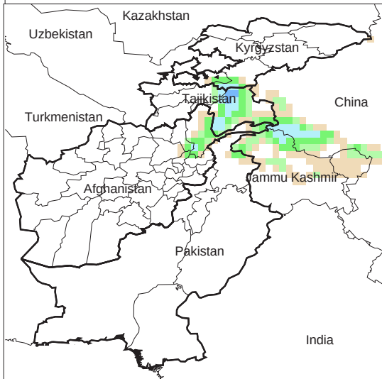
Daily Precip. Forecast for 24 Oct., 2009
