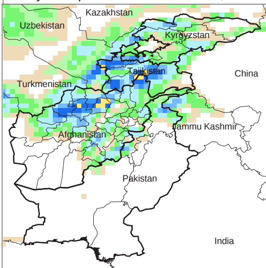
Daily Precip. Forecast for 24 Nov., 2009
