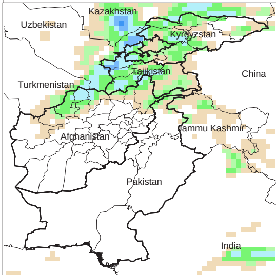
Daily Precip. Forecast for 16 Dec., 2009
