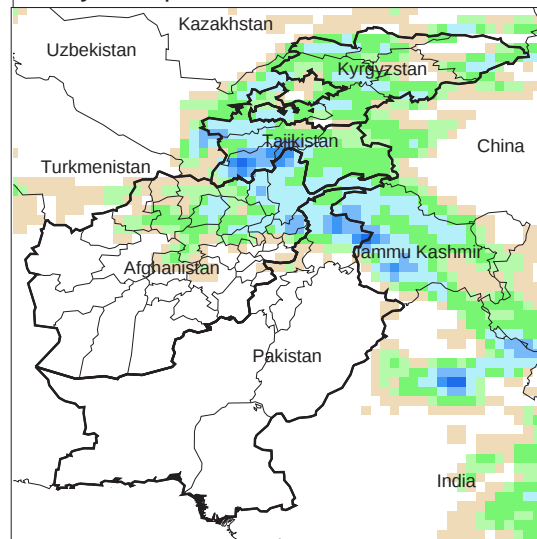
Daily Precip. Forecast for 15 Feb., 2010
