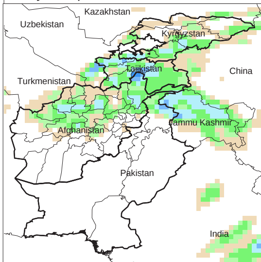
Daily Precip. Forecast for 14 Feb., 2010
